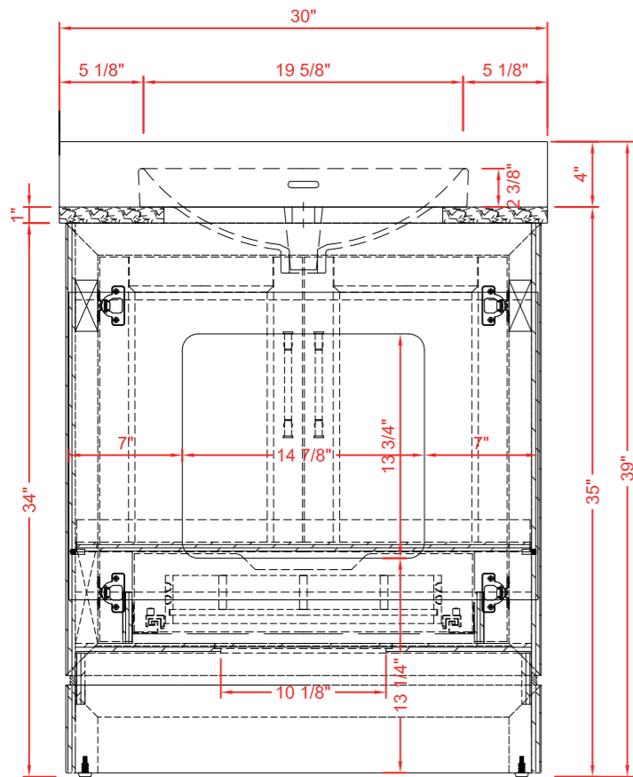
FRONT VIEW
