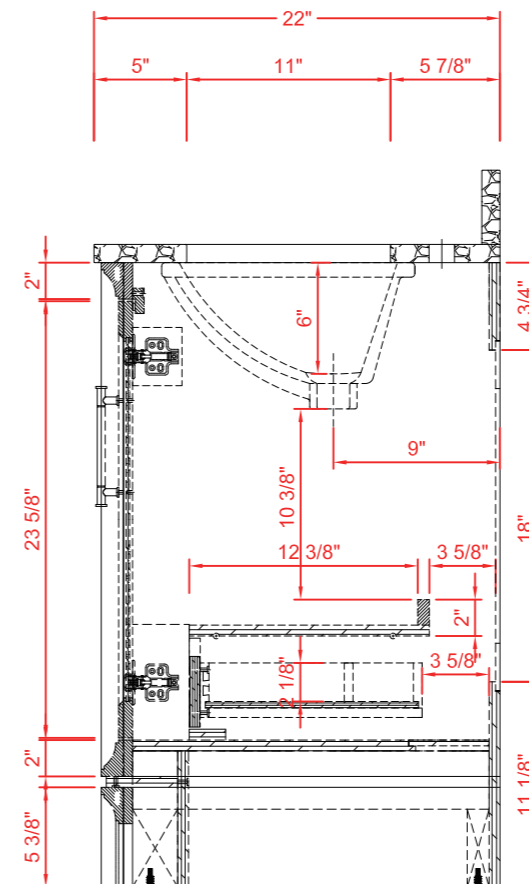
SIDE VIEW
